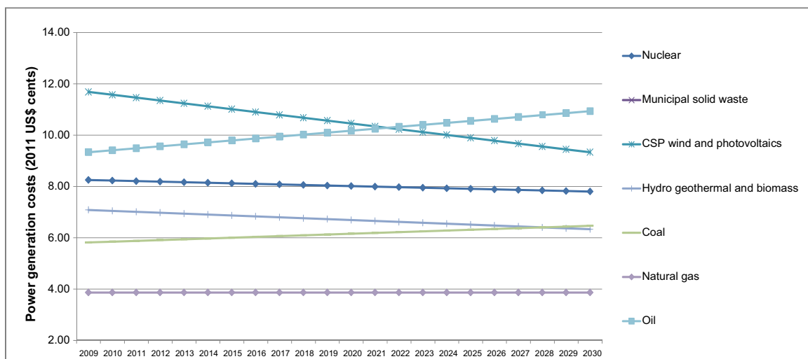
Figure 1. Power generation costs in Africa for each energy source in the reference scenario (2011 cents of US$/KWh). Source: Adapted from Bosetti et al (2006).
