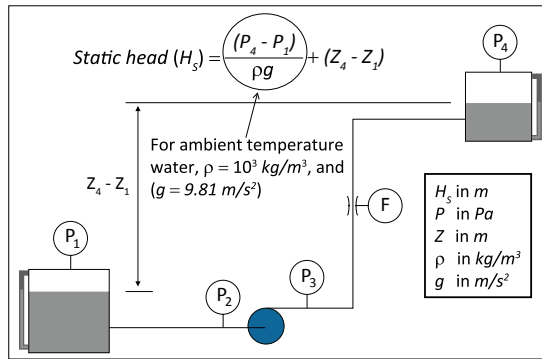
Fig. 13.2. Calculating static head (a)
