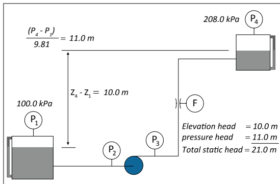
Fig. 13.2. Calculating static head (b)
