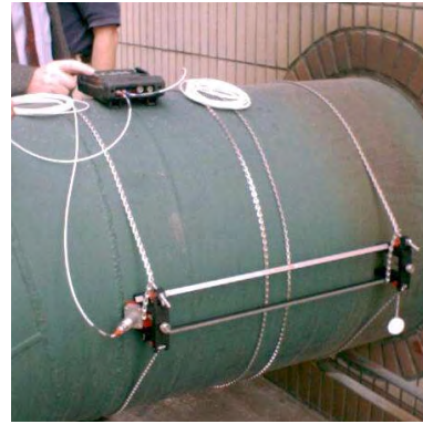
Fig. 12.22. Transit-time ultrasonic flow meter
