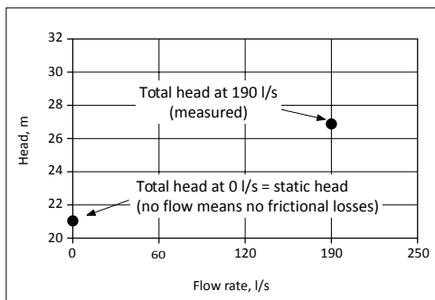
Fig. 13.4. System Curve Development
