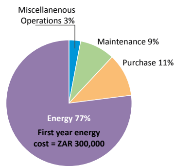
Fig. 1.4. Pump LCC Overview (4380 hours)
