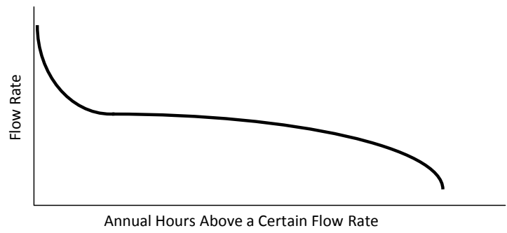
Fig. 2.5. Typical annualized duration curve for a wastewater system
