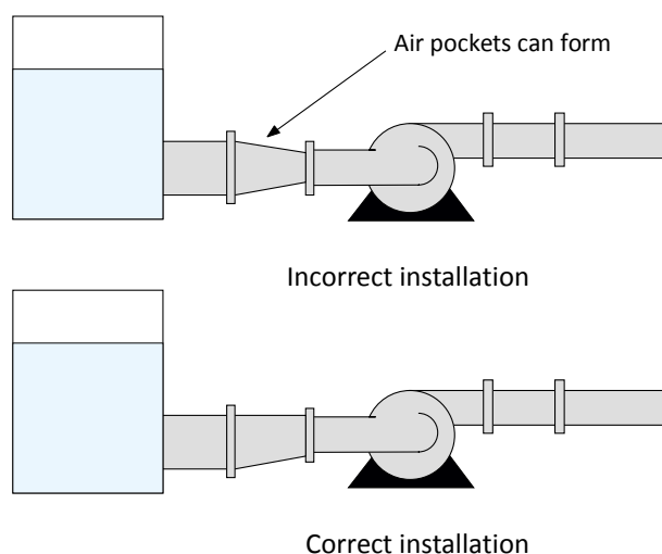
Fig. 6.1. Suction pipe installation
