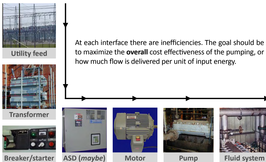
Fig. 2.1. System components
