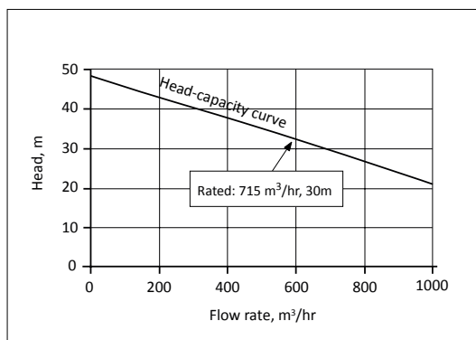
Fig. 5.1. Centrifugal pump head capacity curve
