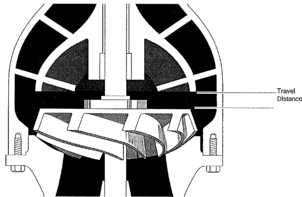
Fig. 6.7. Travel distance for a vertical turbine pump
