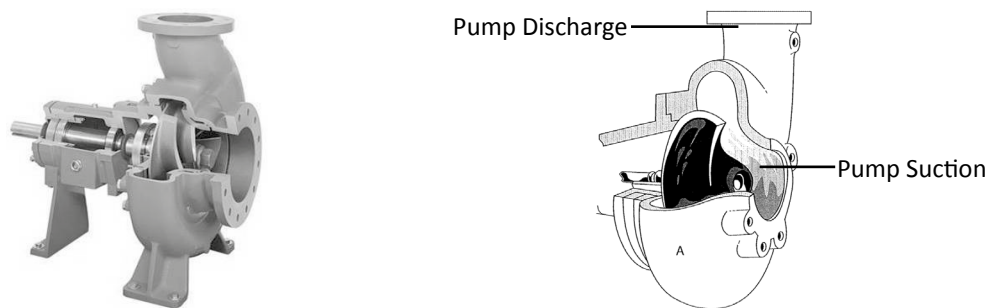
Fig. 3.3. Typical end suction pump
