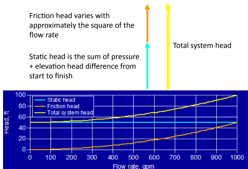
Fig. 12.8. Combination of Static Head and Friction Head
