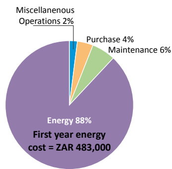
Fig. 1.3. Pump LCC Overview (7000 hours)
