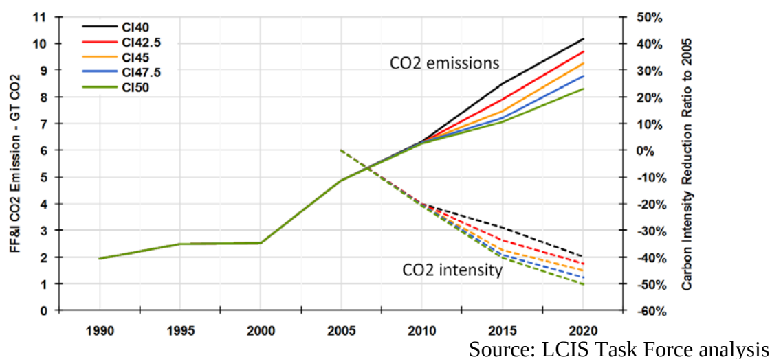
Figure 1-3: Impact of China's carbon intensity reductions on CO 2 emissions
