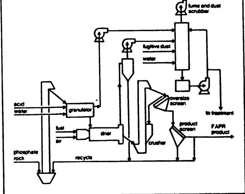
Fig. 5: Single-Step Acidulation/Granulation (SSAG) Process for PAPP
