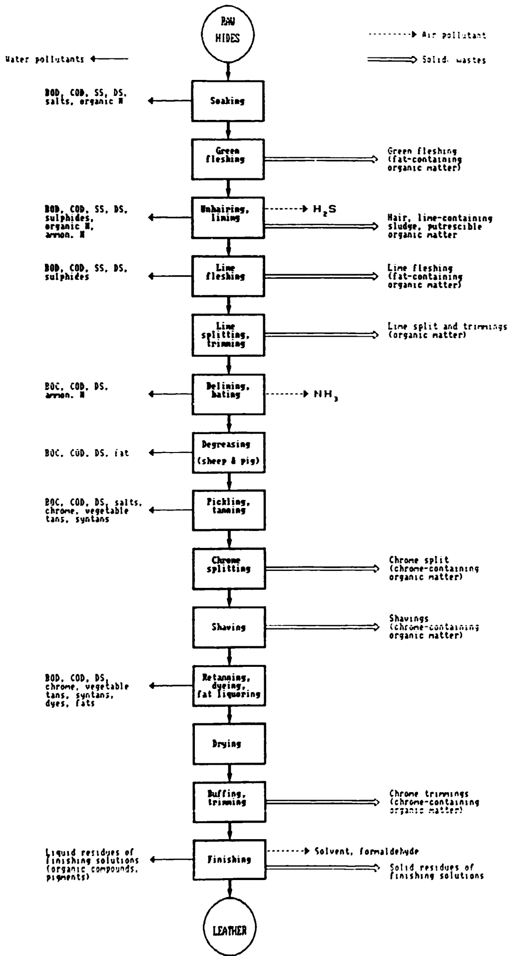
Figure 1. Schematic tanning process Source: UNIDO/UNEP
