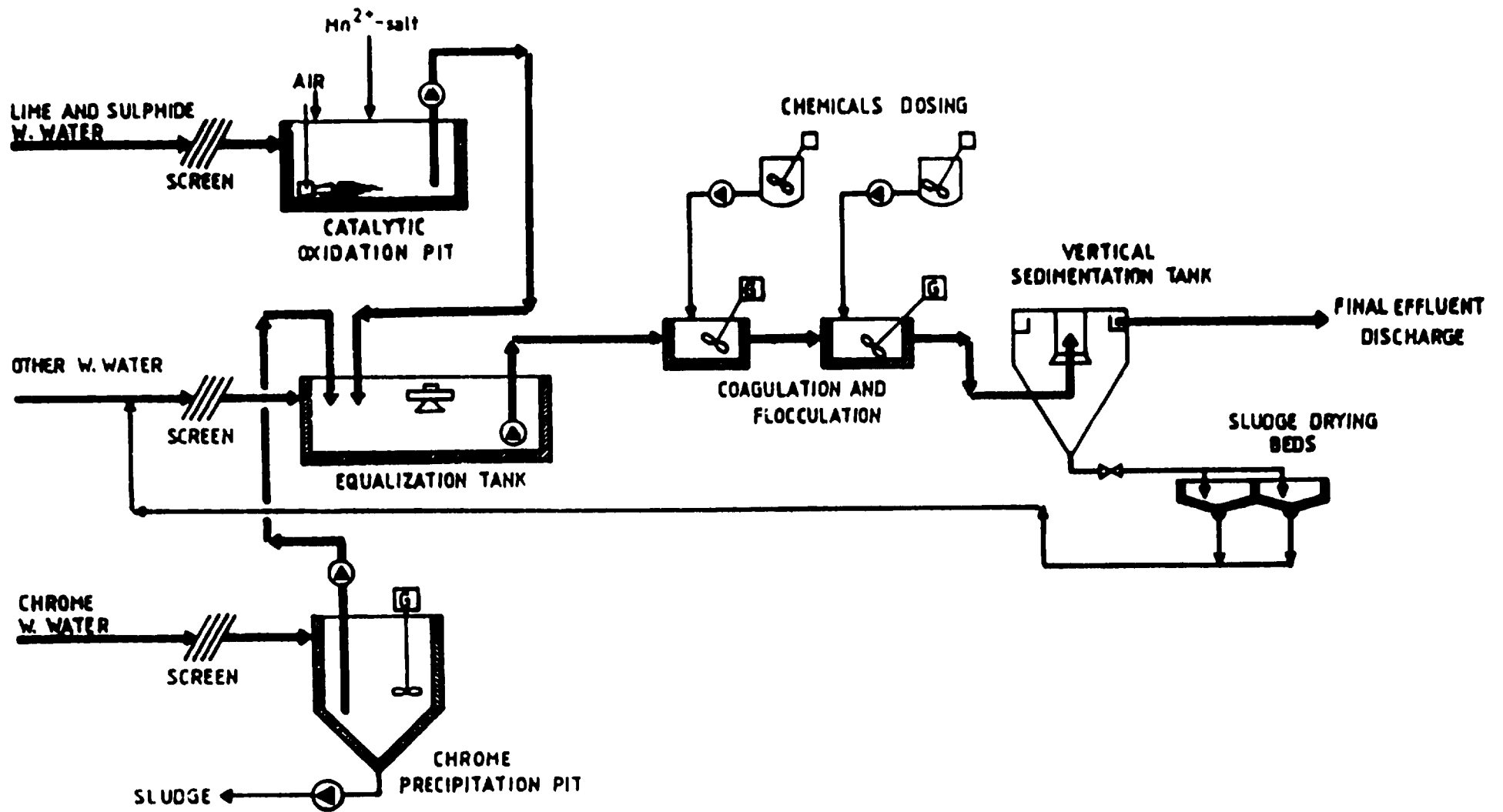
Figure IV. Typical scheme for physical-chemical treatment Source: UNIDO/UNEP
