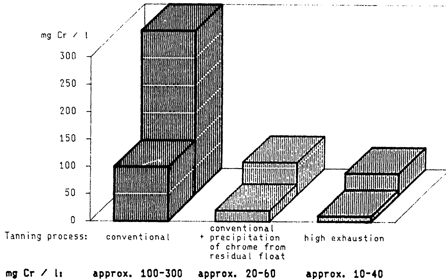
Figure 11. Chrome emissions in tannery effluents
