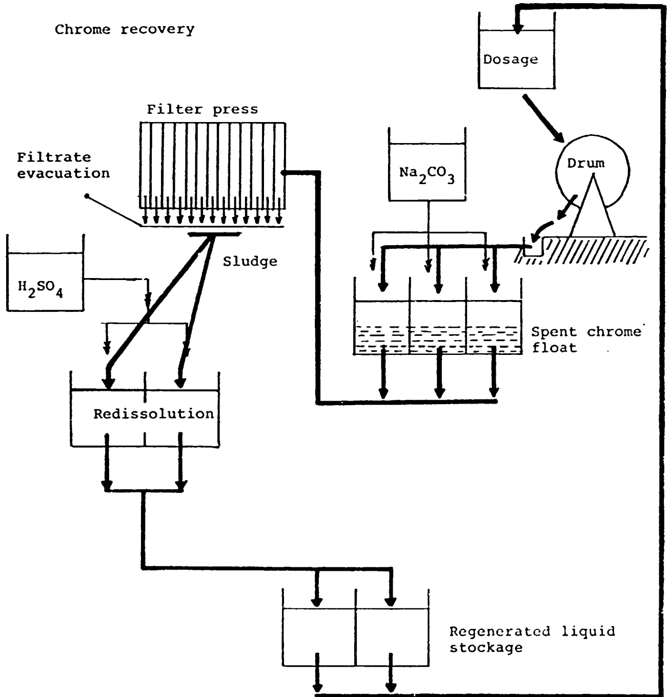
Figure III. Chrome recovery Source: UNIDO
