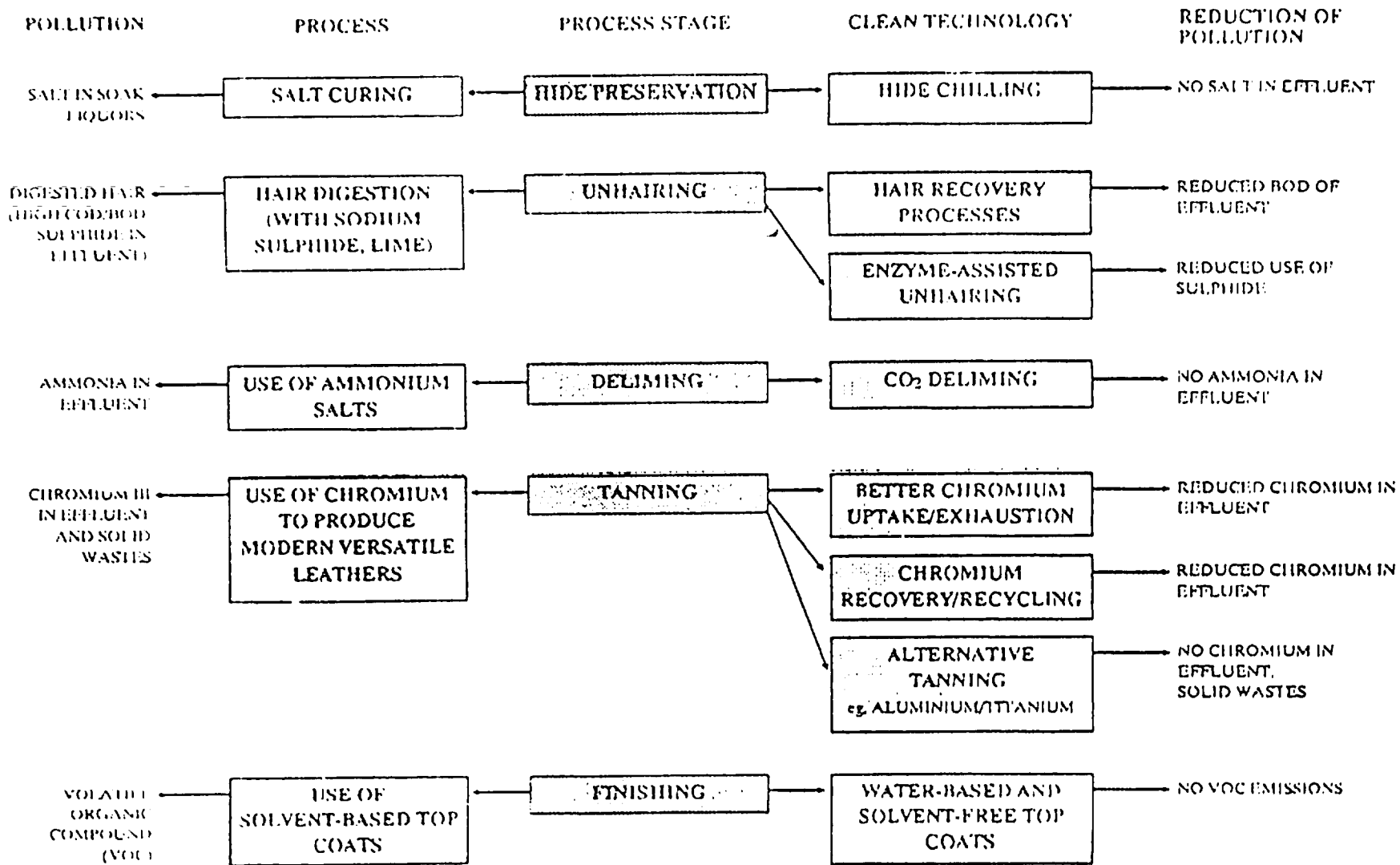
Figure V. Some proposed clean technologies for leather productions
