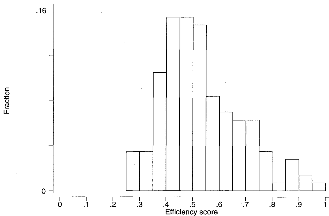
FIGURE 2 THE DISTRIBUTION OF TECHNICAL EFFICIENCY
