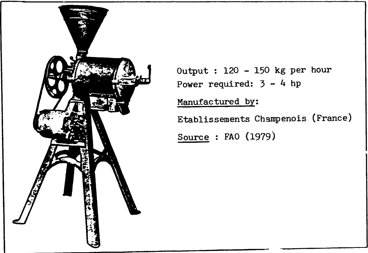
Plate IV.9 Horizontal stone mill
