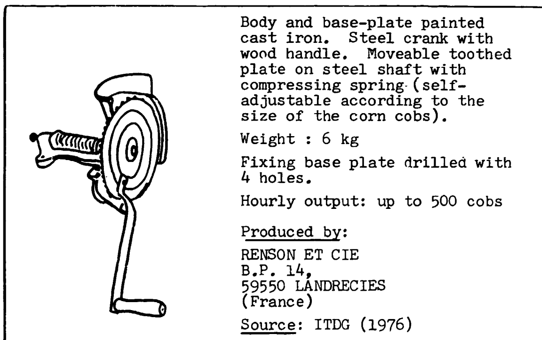
Plate III.2 Hand maize sheller
