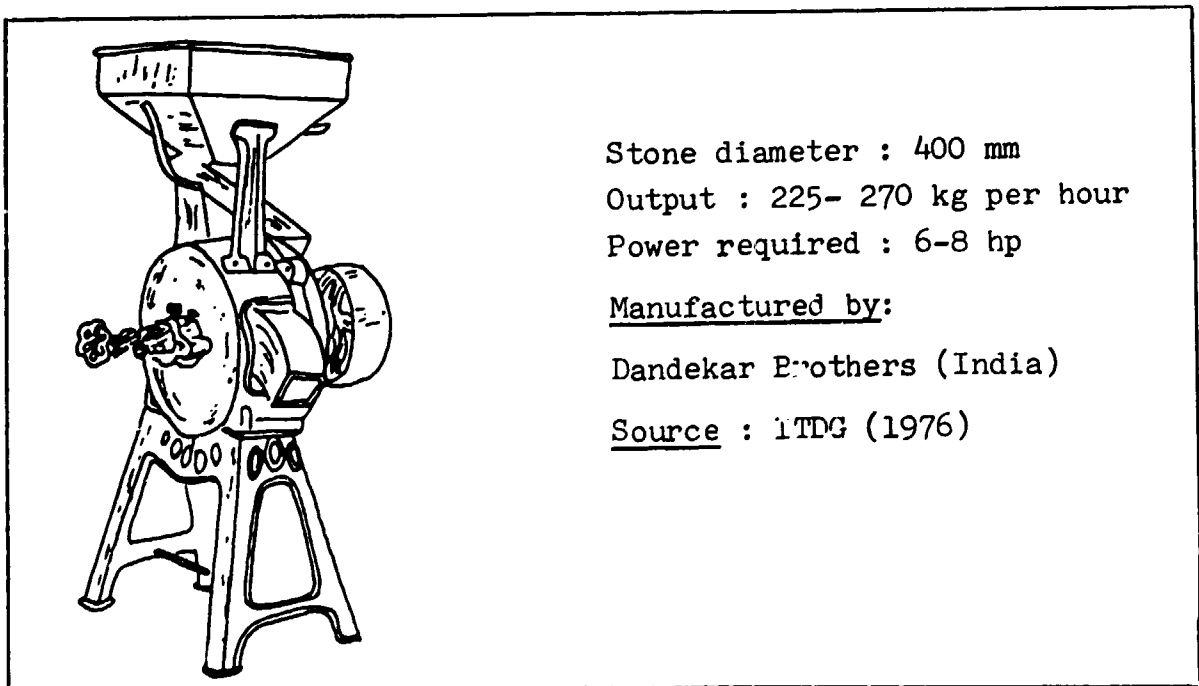
Plate IV.10 Stone mill fitted with natural stones
