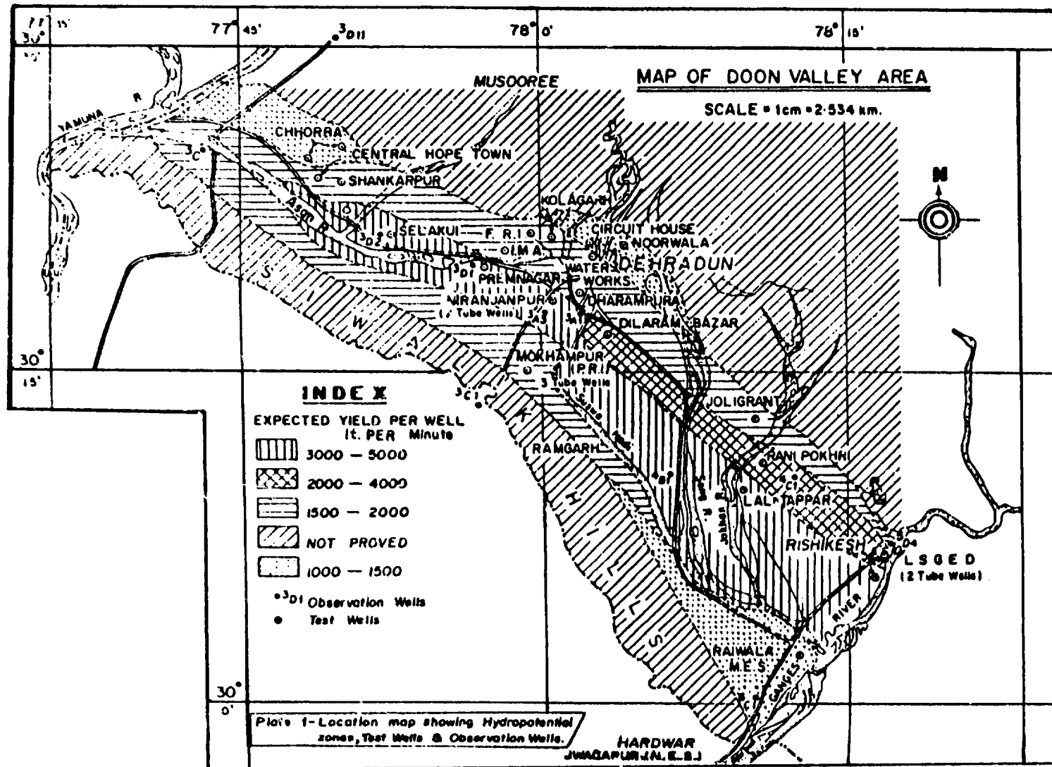
Fig. 7-1 Expected yield per well (litres per minute) in the Doon Valley, based on a survey carried out between 1960 and 1967 by the Exploratory Tubewells Organization, Government of India (Singh, 1973)
