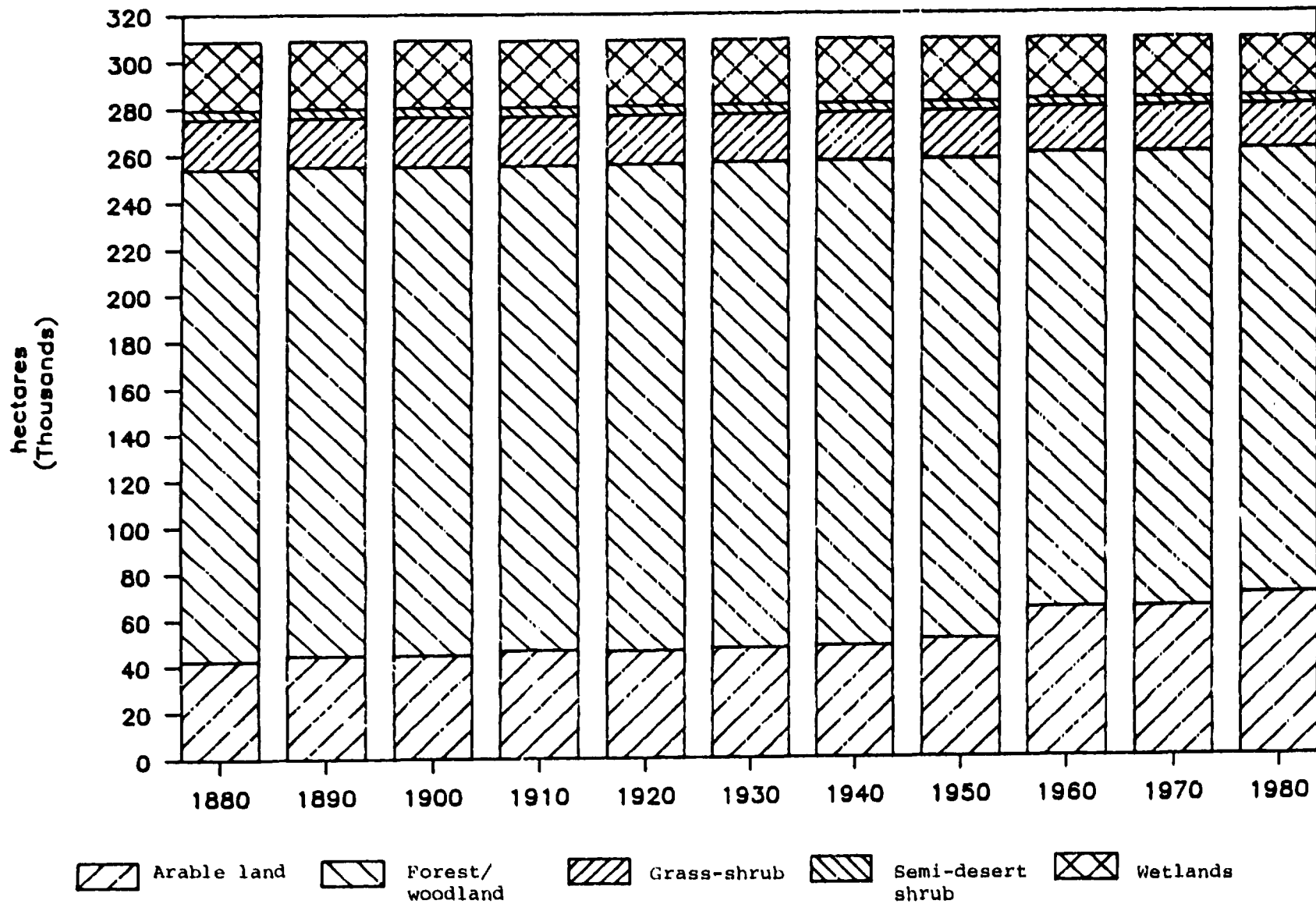
Fig. 5-2 Land Use of Dehra Dun District: 1880 - 1980
