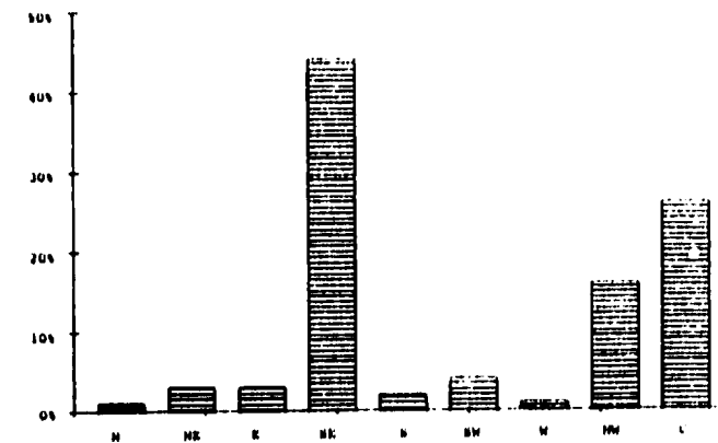
Fig. 6-2a Percentage frequencies of instantaneous wind directions at 0300GMT (0830LST) and 1200GMT (1730LST) in January and July for Roorkee.
