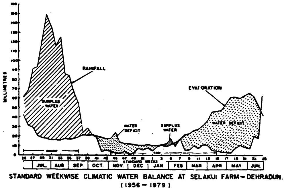
Figure 1 Annual water balance of the Doon valley, comparing precipitation and evaporation
