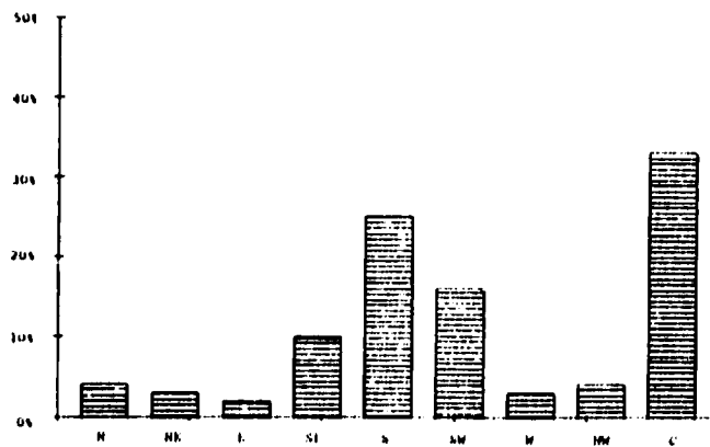
Fig. 6-2c Percentage frequencies of instantaneous wind directions at 0300GMT (0830LST) and 1200GMT (1730LST) in January and July for Mussoorie.
