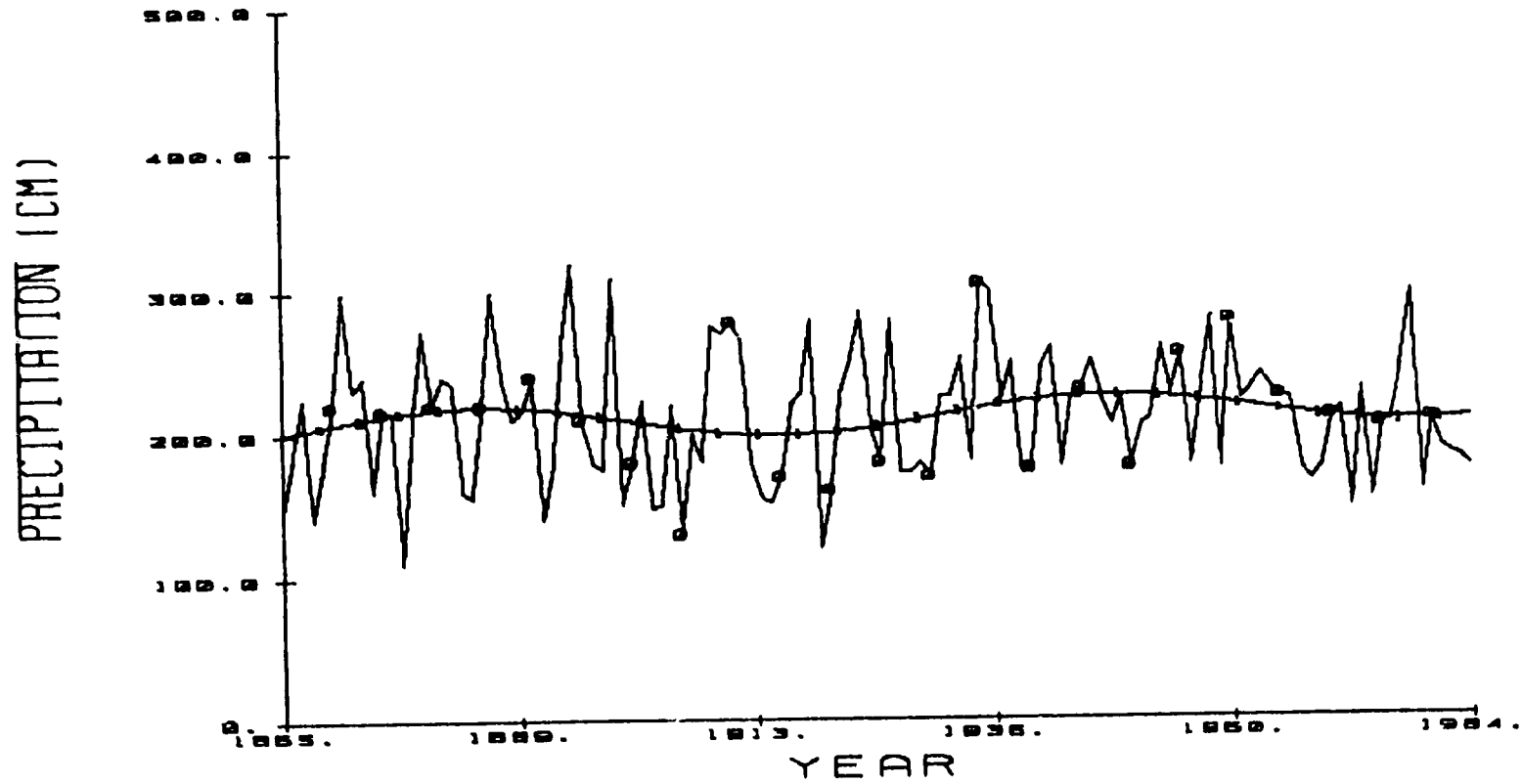
Fig. 6-1 Annual rainfall at the Forest Research Institute, Dehra Dun. A best-fitting curve is included.
