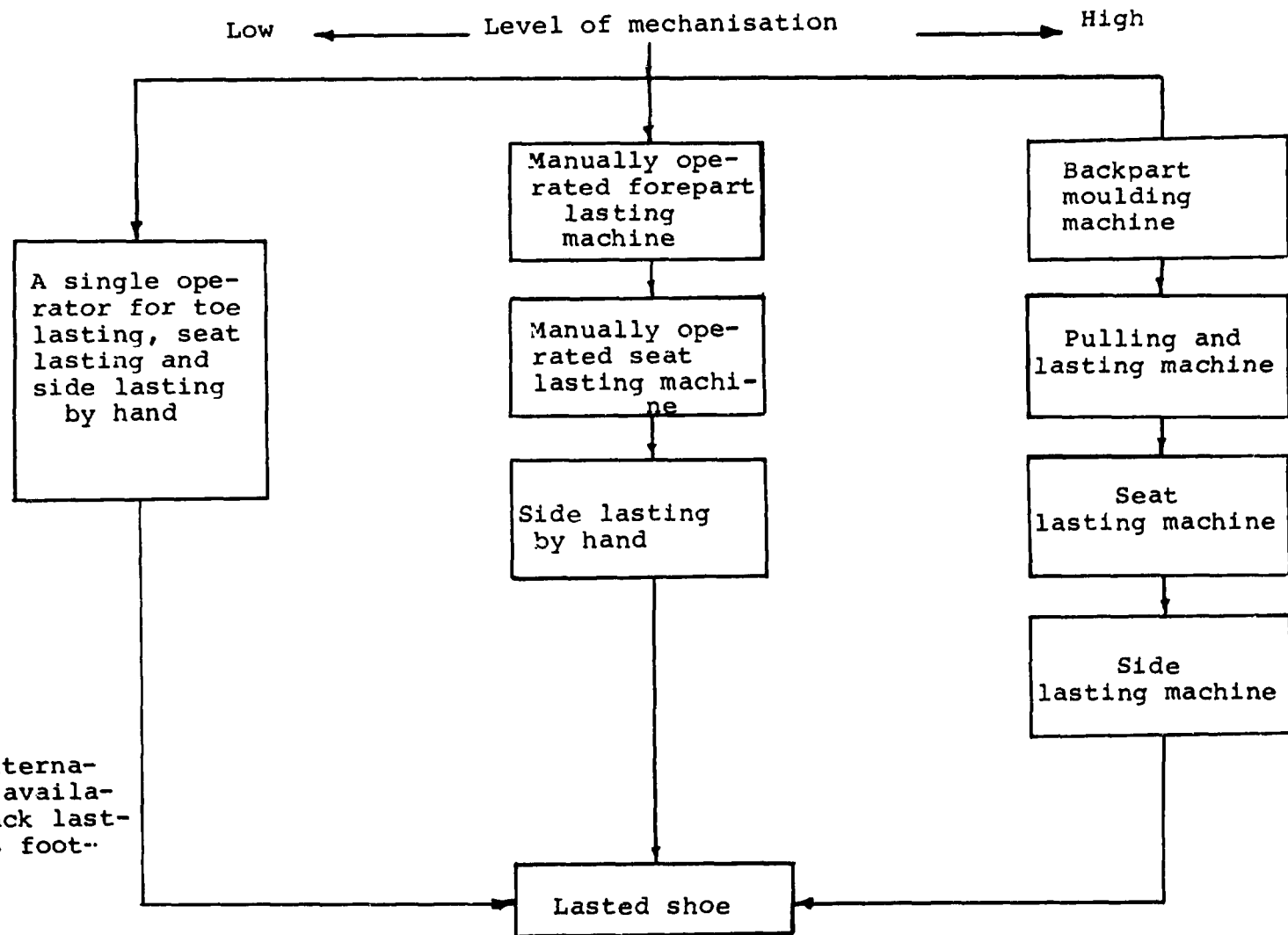
Figure II.10 Alternative cement-lasting sequences
