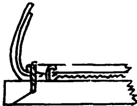
Type 3. Tack-lasted, machine-sewn sole
