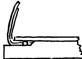
Type 4. String-lasted, moulded-on sole
