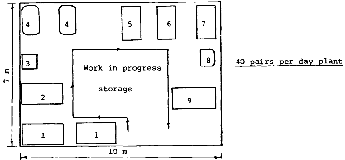
Figure II.14 Layout of production areas for type 1 footwear - 40 and 200 pairs per day
