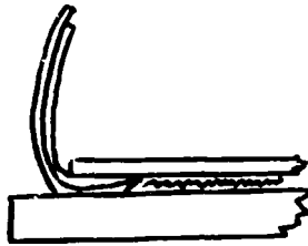
Types 1 and 5. Cement-lasted cemented-on sole
