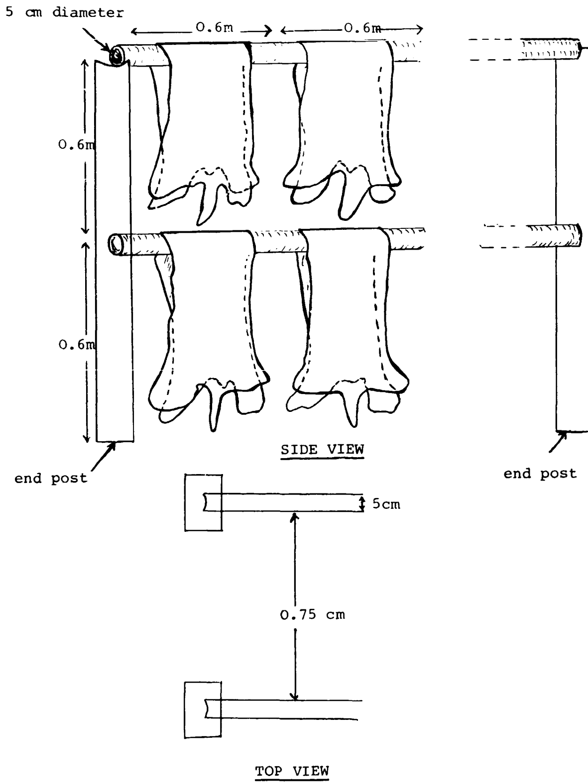
Figure VI.9 Drying rails for oiled skins
