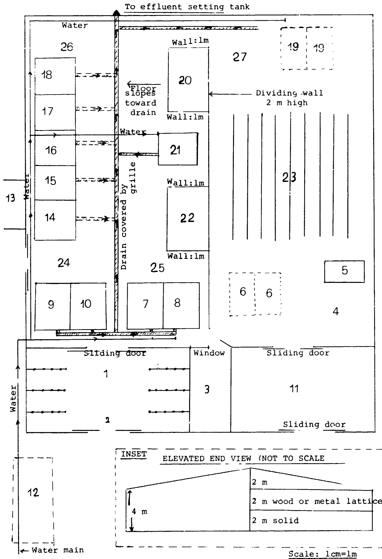
Figure V.8 Floor plan for vegetable tanning of 20 hides per day
