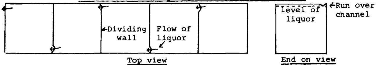
FIGURE V.3(a) Procedure for 4-day vegetable tanning of hides
