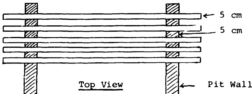
Figure V.1 Suspension of hides in pits
