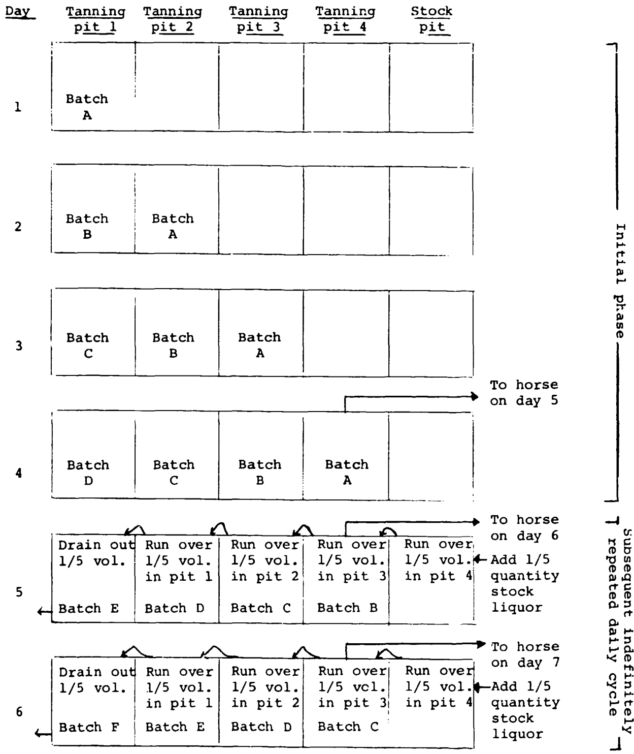
FIGURE V.3(a) Procedure for 4-day vegetable tanning of hides
