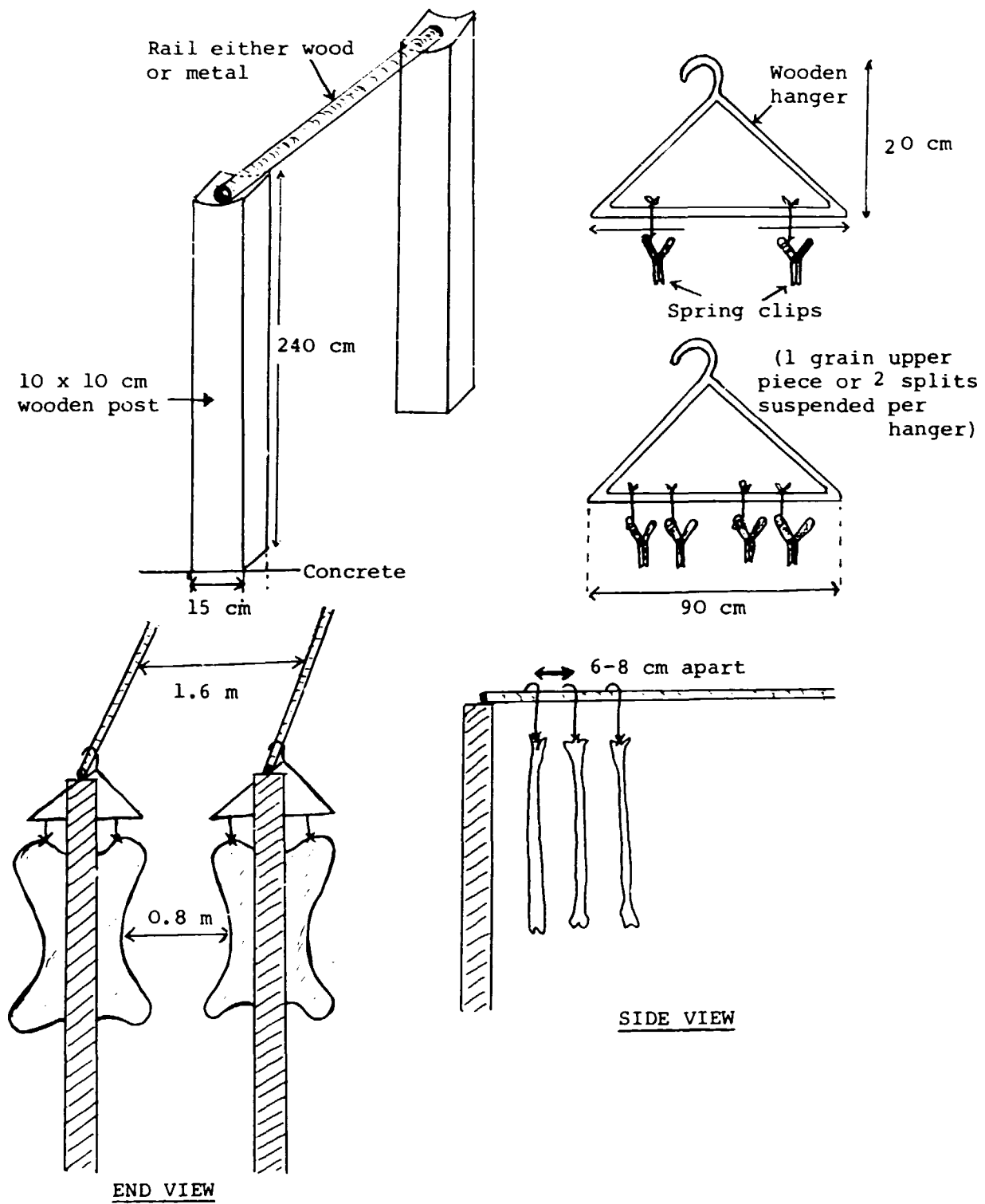
Figure IV.10 Rails for hanging leather
