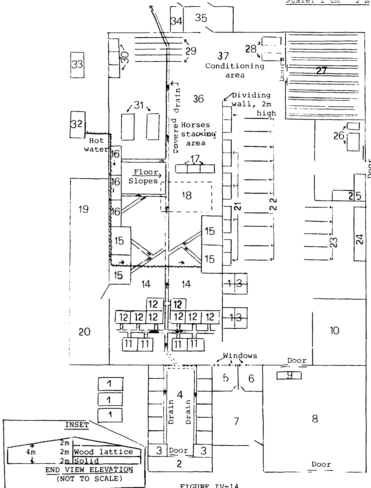
FIGURE IV-14 Floor plan for low investment cost tannery Handling 200 hides per day (ML Project)
