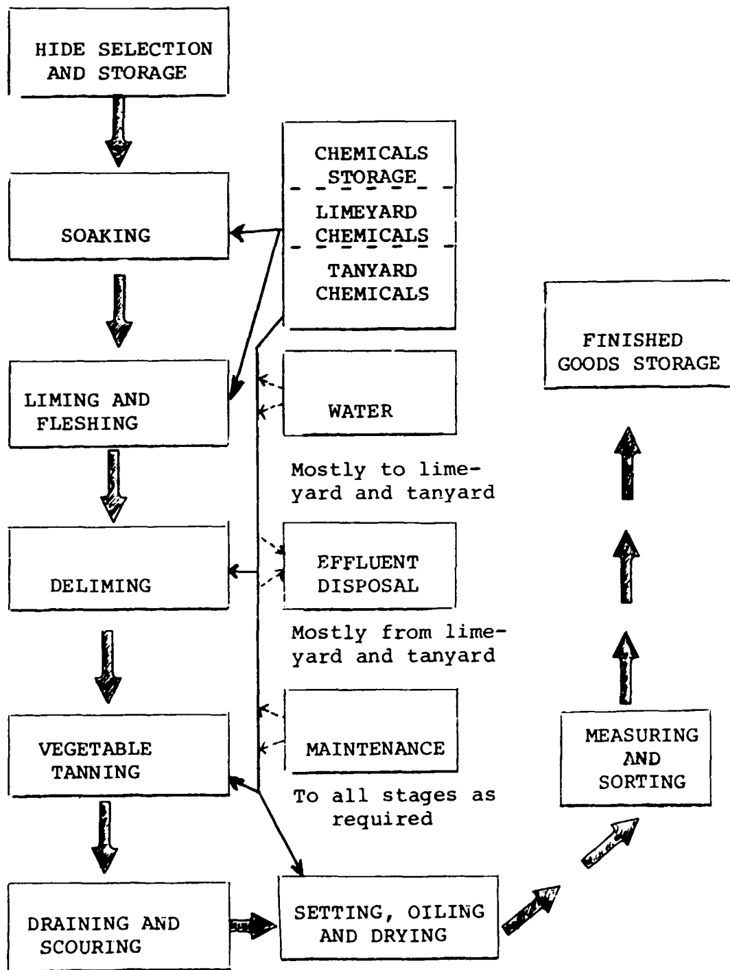
Figure V.7 Simplified diagram for the vegetable tanning of hides (MS-hides project)
