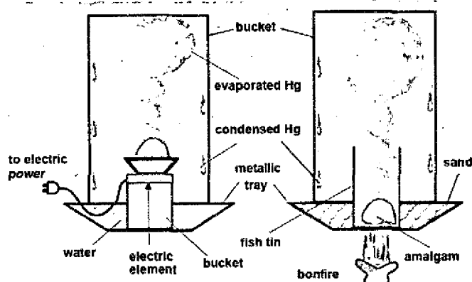
A home-made retort from China (left) dan Papua New Guinea (right)
