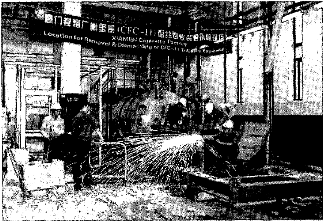
Dismantle Scene (The CFC-11 equipment was dismantling)
