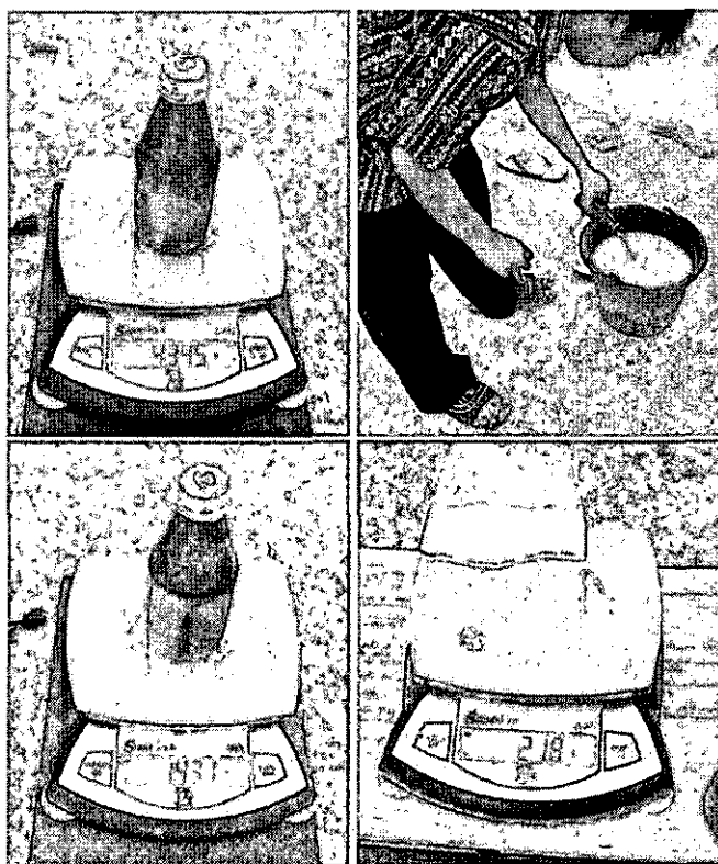
Figure 4-8 directly weighing and calculating amounts of mercury consumed during the amalgamation process and gold refining. This method revealed that on average for the region 1.5 units of mercury are consumed per unit of gold recovered and that 30% of the mercury is lost to the tailings and the rest lost to the atmosphere when heated later in the gold shops to produce the gold.
