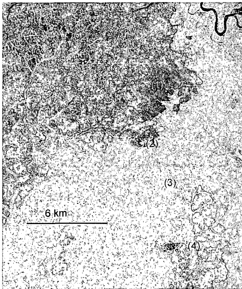
Figure 4-10 Change Detection Map of the Galangan sand fields derived from multiple PALSAR scenes collected between June and November 2006 (ground truth was simultaneously collected). Colors correspond to degrees of change in the four month period between June and September (Green = moderate, yellow = large, red = extreme). At site (1) some 2000 hectares appear totally vacant – no change. A closer look at Figure 4-2, taken across this region, reveals that this is indeed the case - the mine fields here have been completely abandoned. Aerial photographs taken at locations 2, 3 and 4 are shown and explained in Figure 4-11, Figure 4-12, and Figure 4-13.
