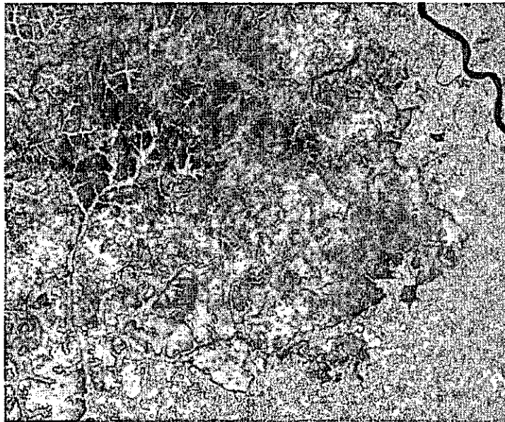
Figure 4-9 PALSAR L-band RADAR scene of Galangan, ground resolution is 12.5 meters. The lighter areas on along the east and southern edges remain forested (high stem volume increases backscatter making these areas brighter) while the dark areas (low backscatter) result from cleared land, ground and standing waters as well as ASM.
