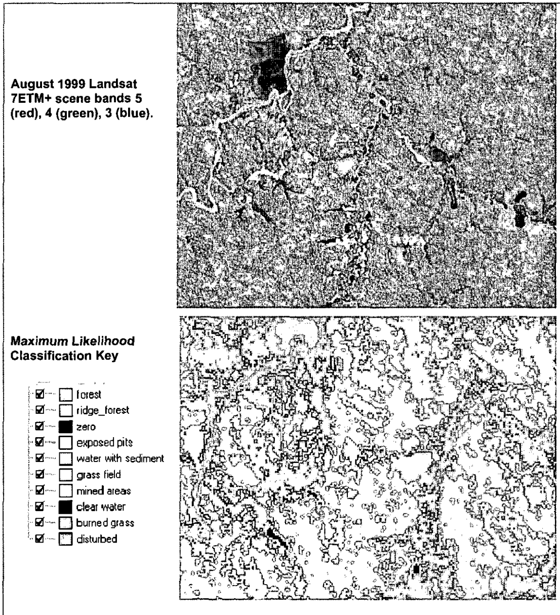
Figure 5-3 Subset of Landsat 7 ETM+ Composite Image (Bands 5,4,3), August 1999 (upper) and corresponding supervised classification result (lower) used to delineate the areal extent of ASM.
