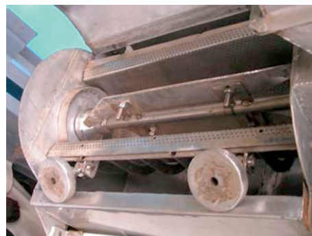
Fig. 5.18. Pulping mechanism
